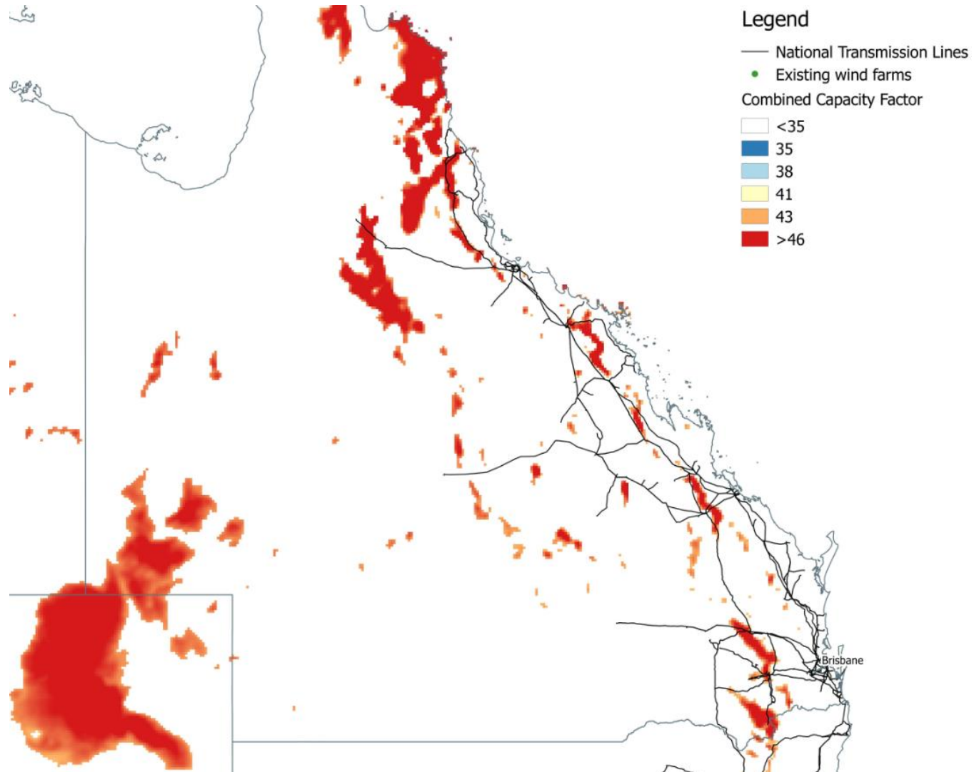
Figure 62 Queensland combined wind + solar capacity factor (Method 1; poor wind and poor solar resource locations removed)
