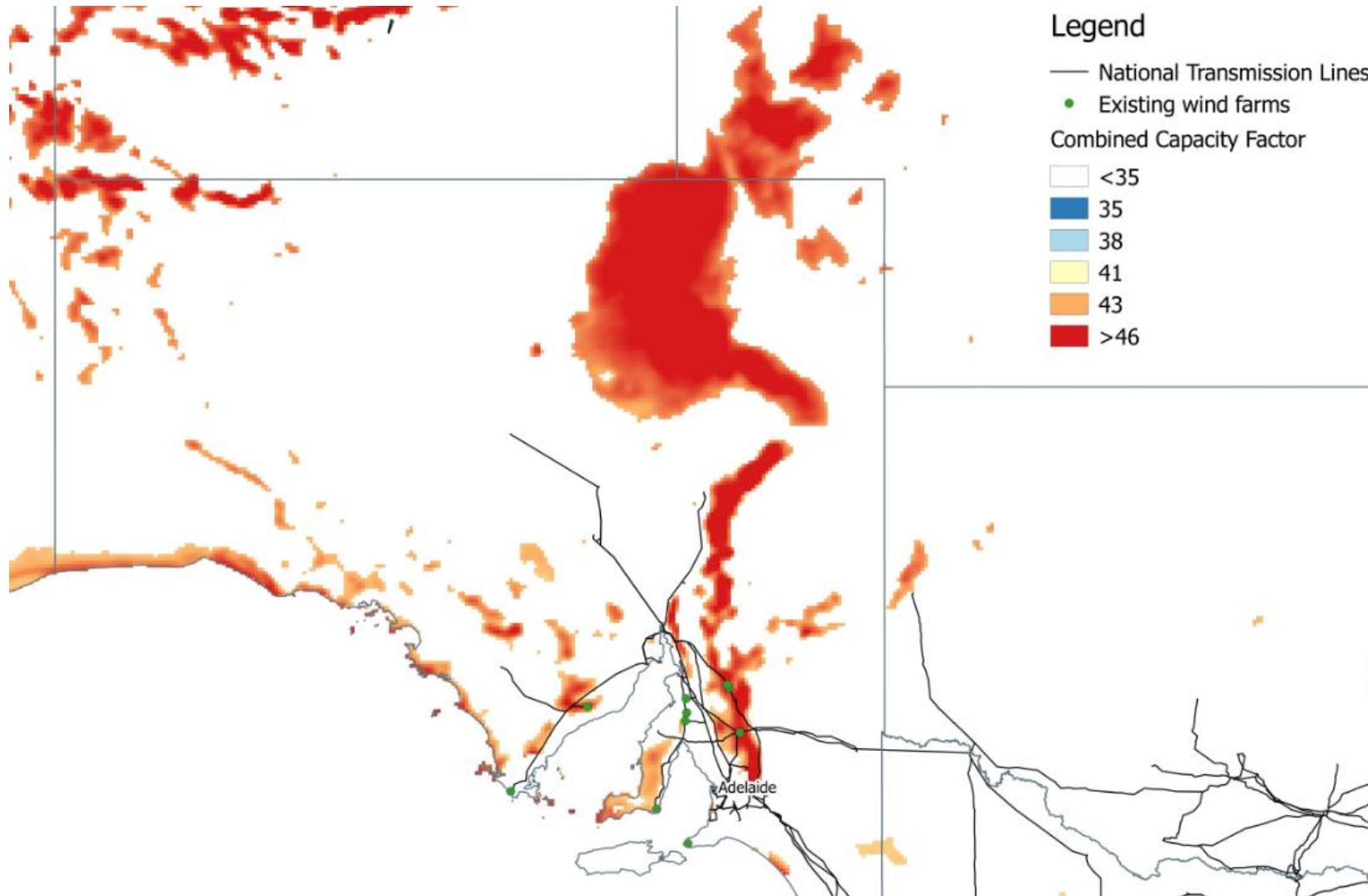
Figure 63 South Australia combined wind + solar capacity factor (Method 1; poor wind and poor solar resource locations removed)
