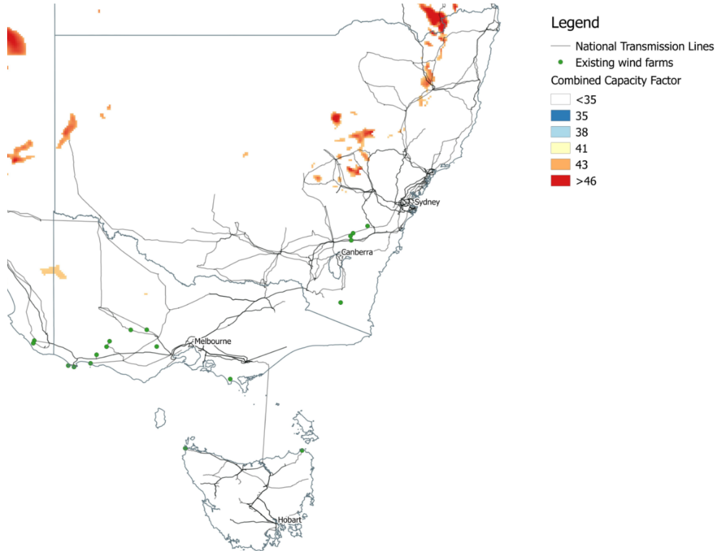
Figure 61 South eastern Australia: combined wind + solar capacity factor (Method 1; poor wind and poor solar resource locations removed)
