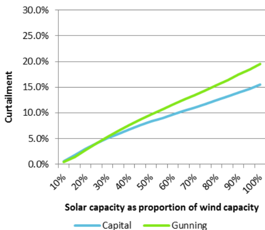
Figure 40 Solar generation curtailment at each in NSW
