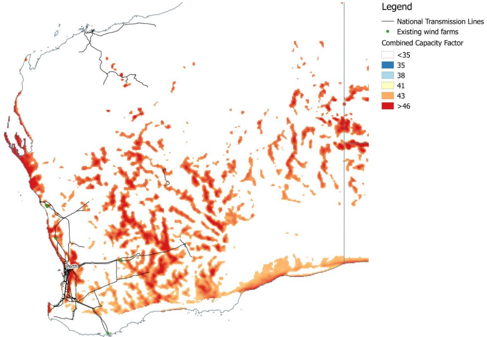
Figure 64 Western Australia combined wind + solar capacity factor (Method 1; poor wind and poor solar resource locations removed)
